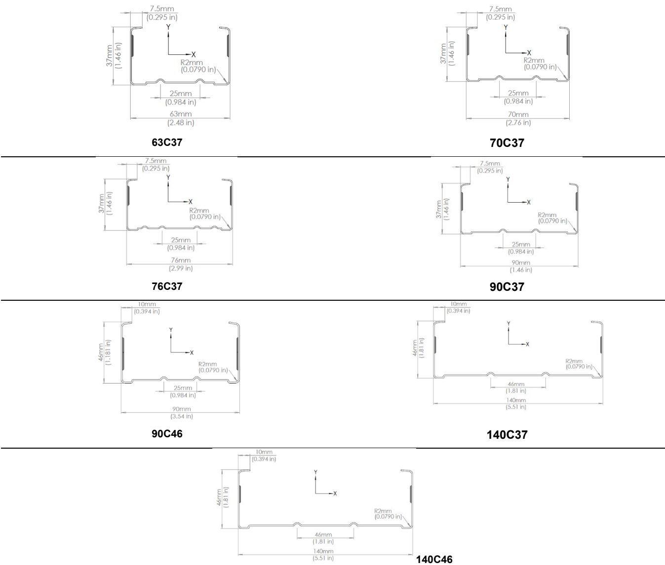
FIGURE 1 – COLD FORMED STEEL FRAMING MEMBER SECTIONS
